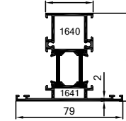
64-5566-5567 1.741 kg/m
