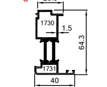
64-3640-3542 2.430 kg/m
