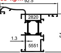
64-2820-5551 1.538 kg/m
